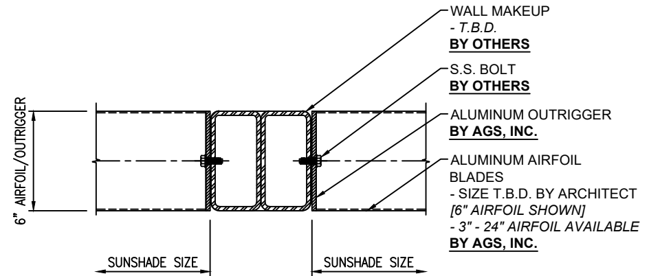
STANLEY SERIES "Arizona" CONNECTION DETAIL
