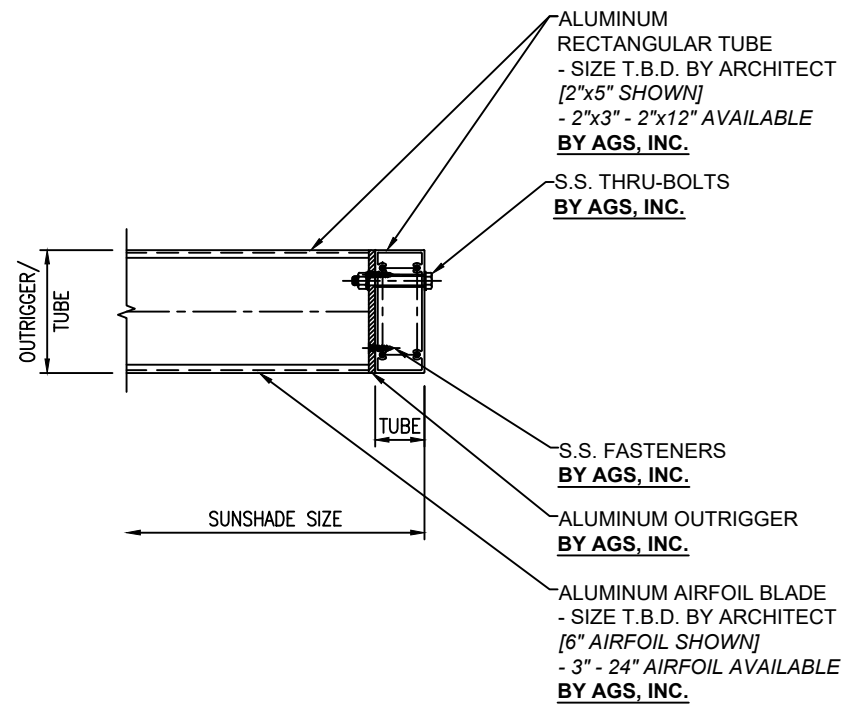
STANLEY SERIES "Colorado" SUNSHADE SECTION - END CONDITION
