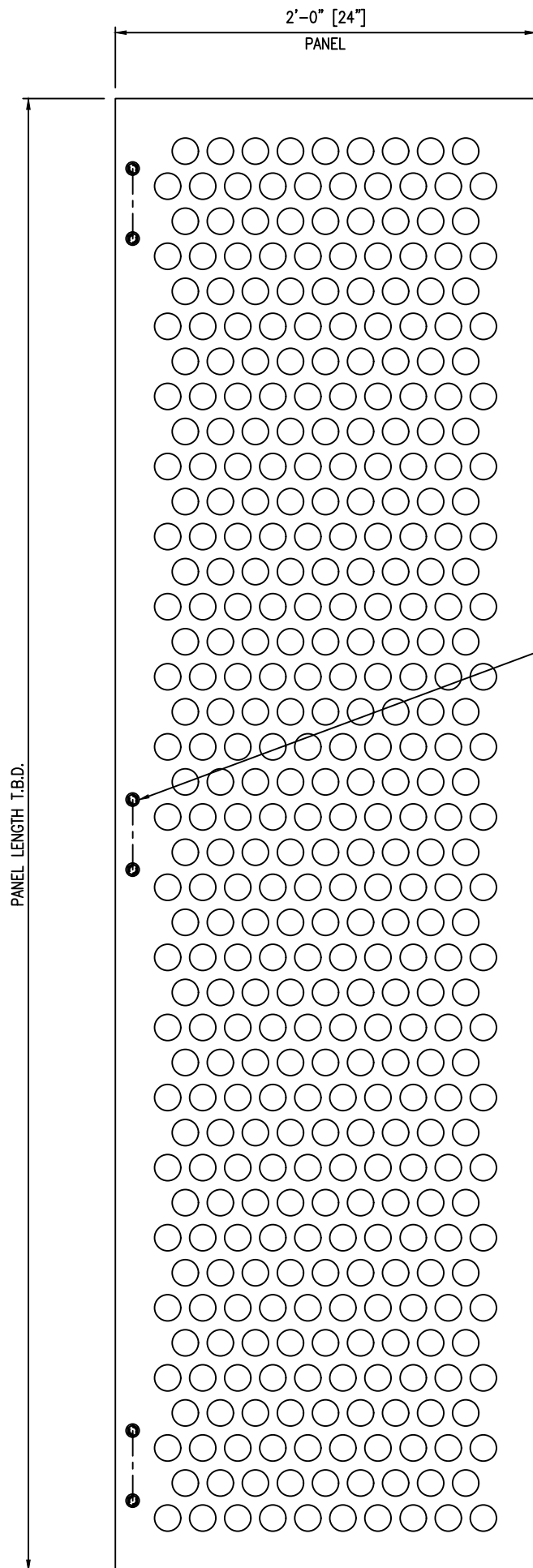
STANLEY SERIES - "Montreal" SUNSHADE SECTION
