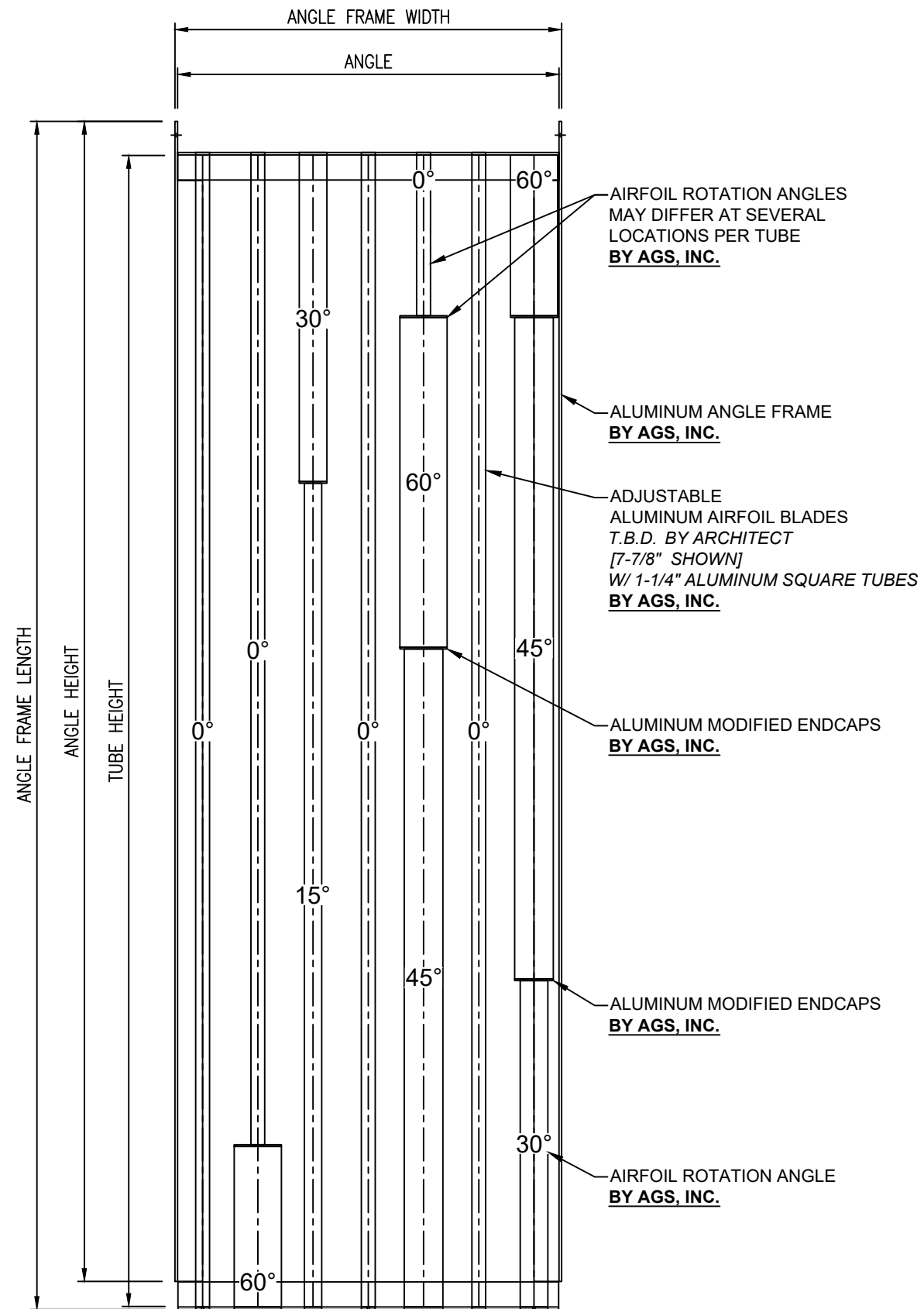
STANLEY SERIES "New York" SUNSHADE ELEVATION
