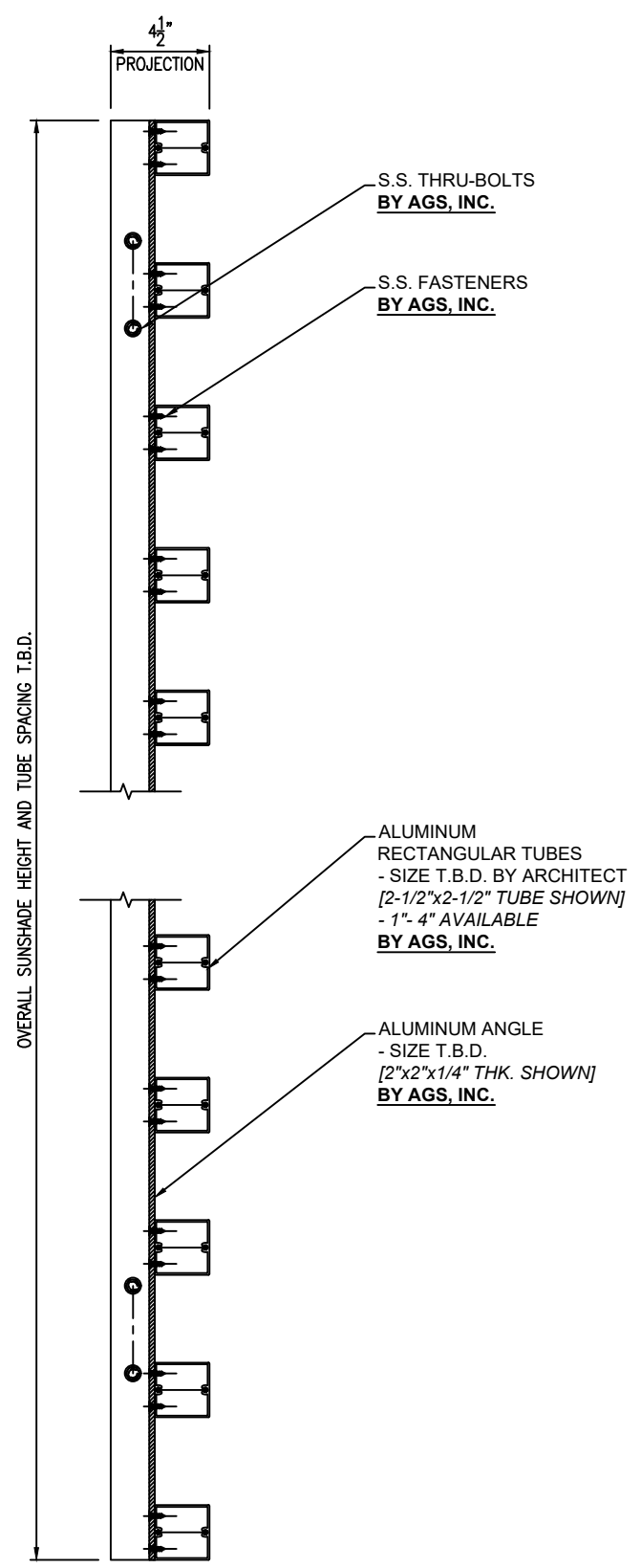
STANLEY SERIES "Vancouver" SUNSHADE SECTION
