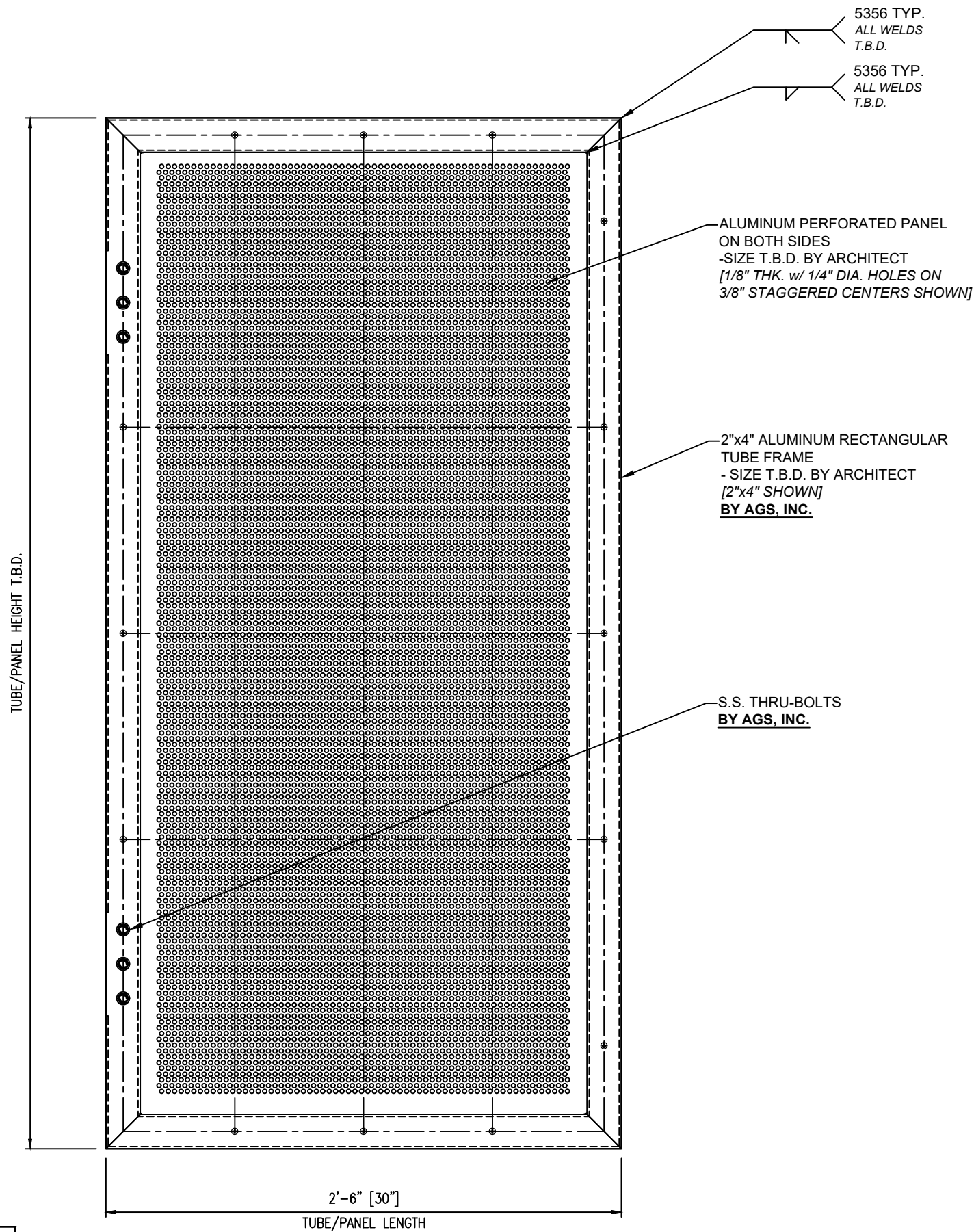
STANLEY SERIES "Vegas" SUNSHADE SECTION
