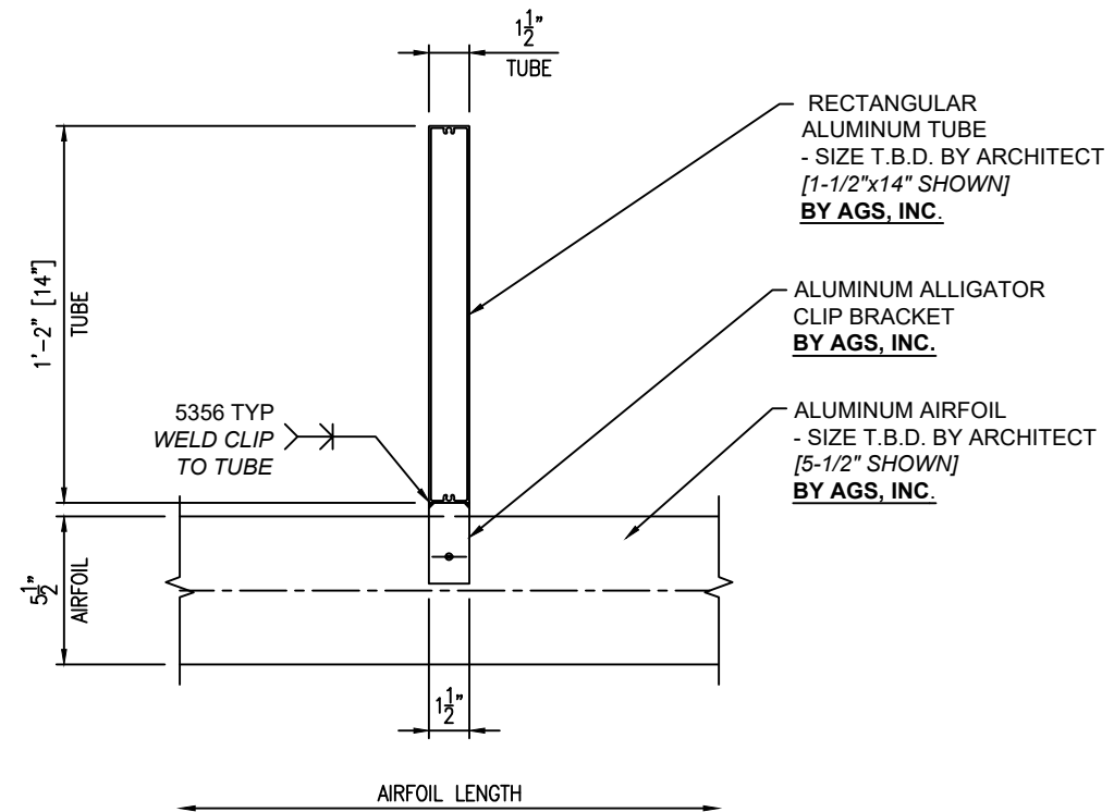
STANLEY SERIES "Pittsburgh" CONNECTION DETAIL
