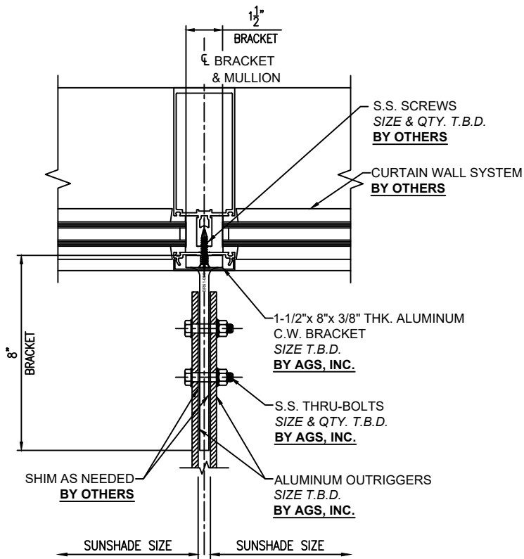
01 PLAN DETAIL AT VERTICAL MULLION SCALE: 6" = 1'-0"
