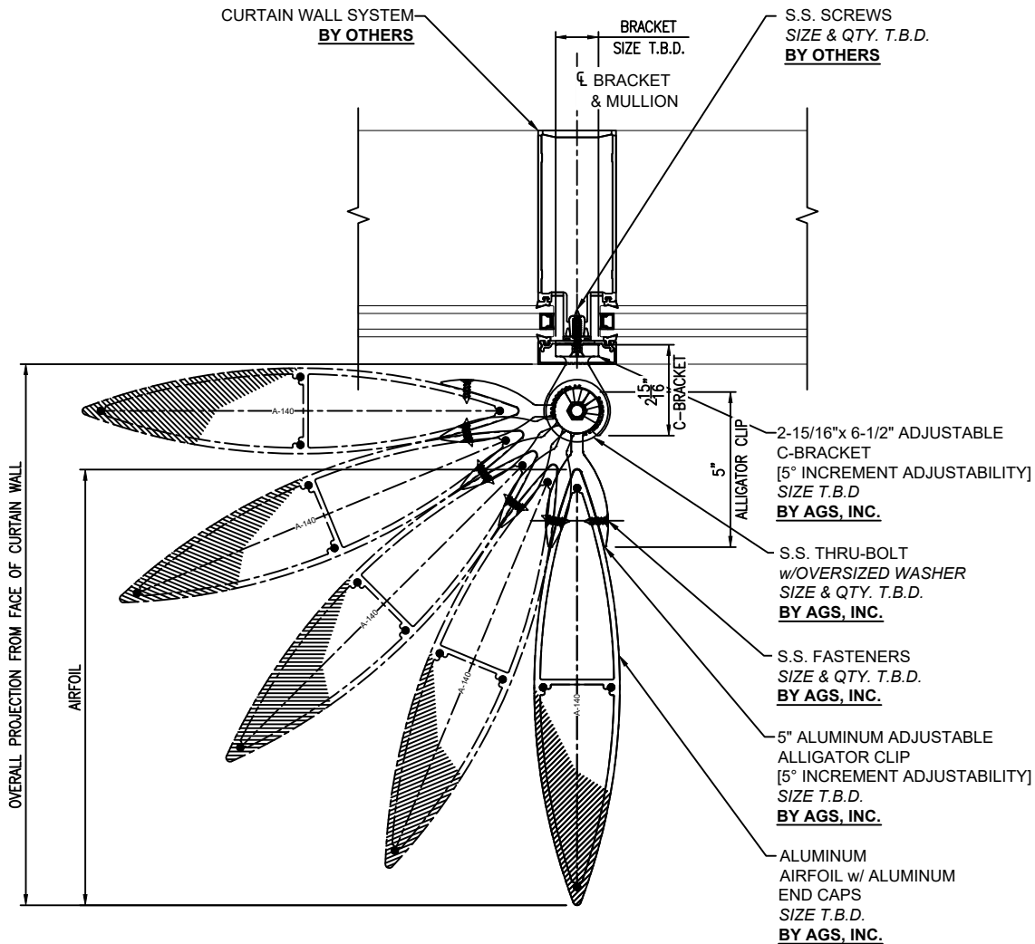
01 PLAN DETAIL AT VERTICAL MULLION SCALE: 6" = 1'-0"
