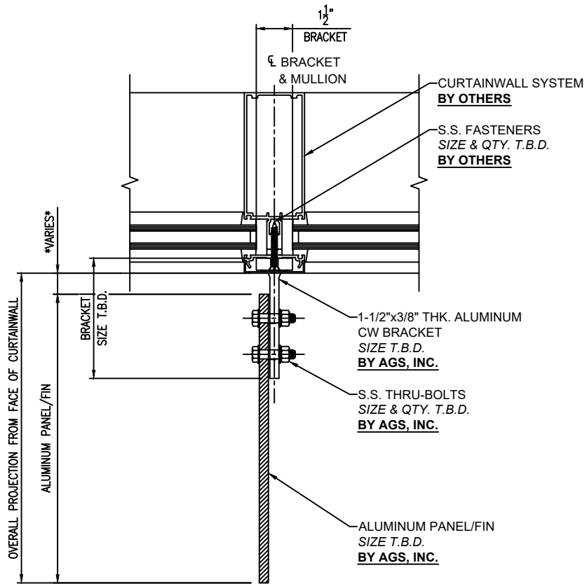
01 PLAN DETAIL AT VERTICAL MULLION SCALE: 6" = 1'-0"
