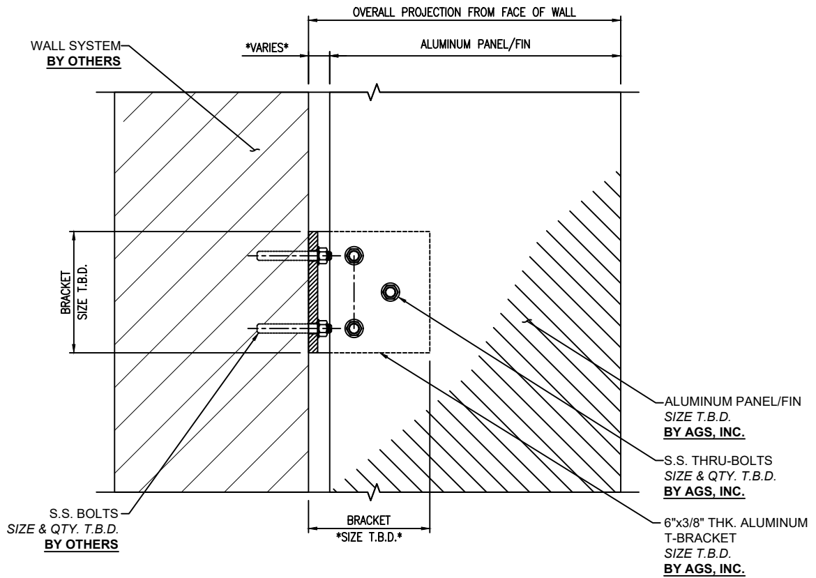
02 SECTION DETAIL SURFACE MOUNT SCALE: 6" = 1'-0"
