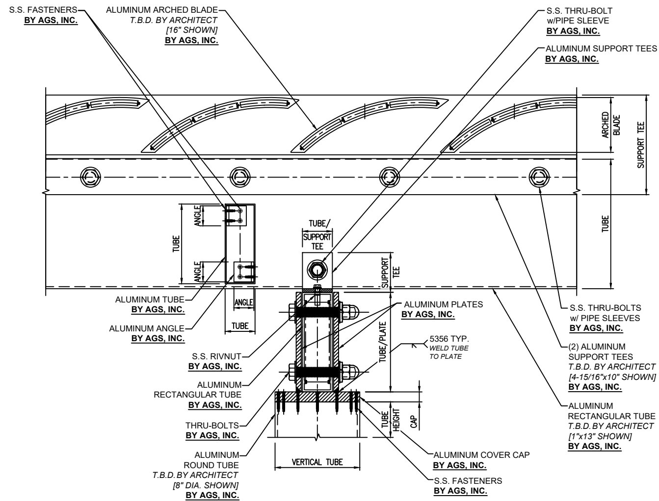
WINDY CITY SERIES "Marina City" CONNECTION DETAIL - SECTION VIEW
