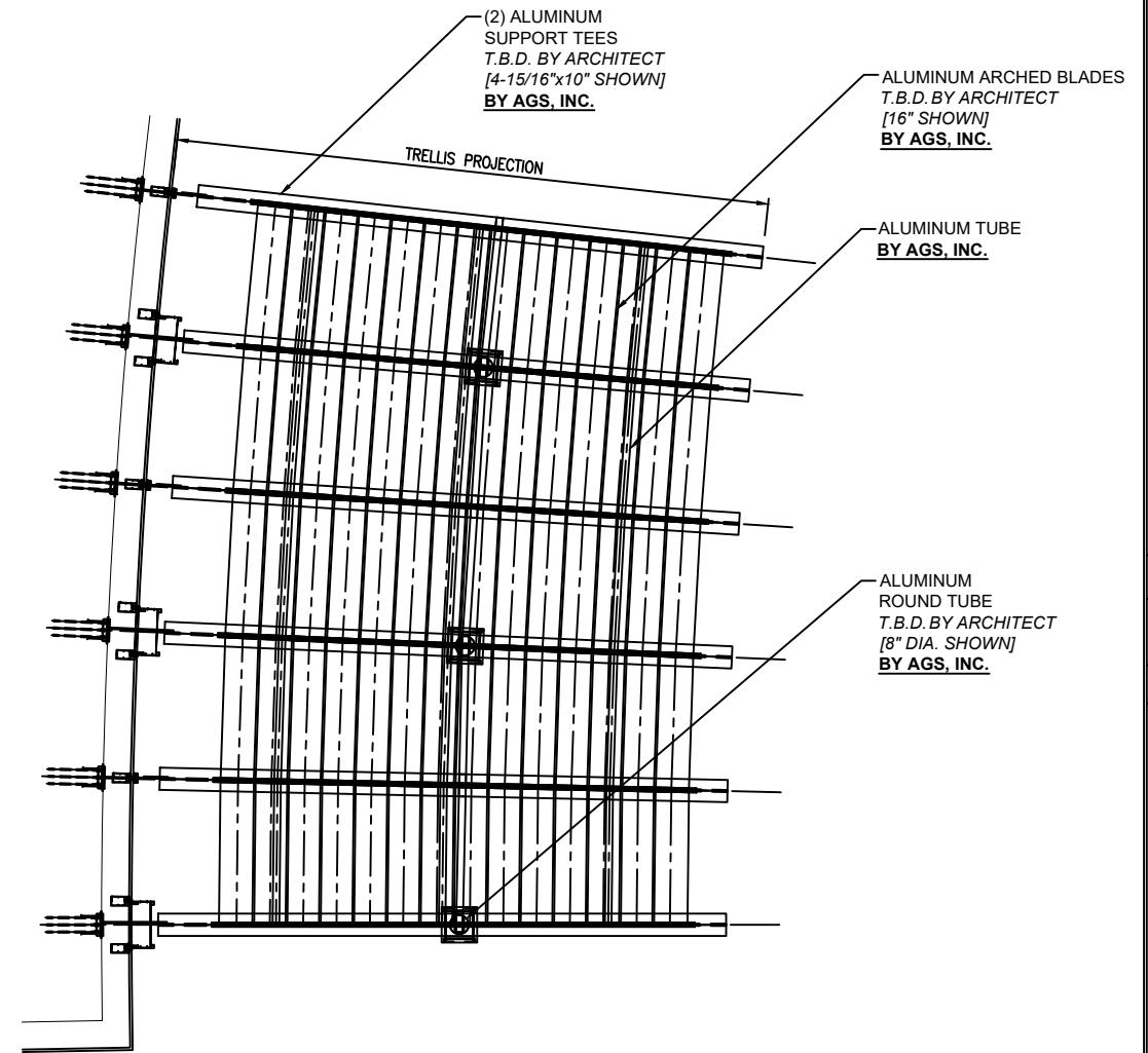
WINDY CITY SERIES "Marina City" TRELLIS PLAN VIEW
